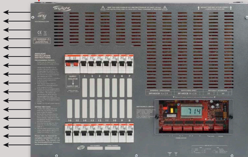
DP1602CB 16 channel dimming/switching pack with Anylight Interface fitted
