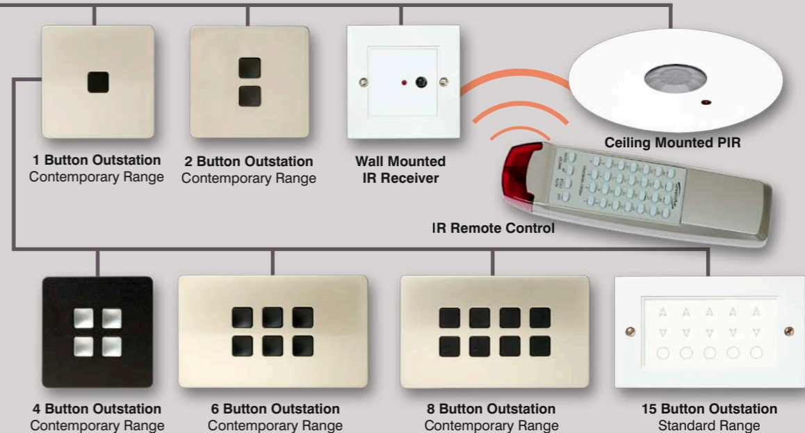
Two wire connection to outstations
